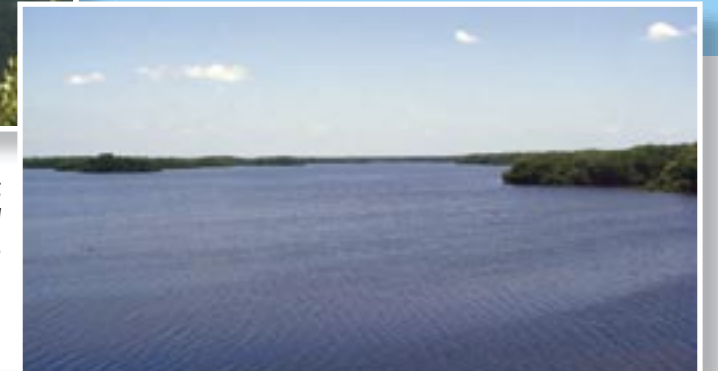
Above photo depicts extent of current algae bloom. Photo to right shows conditions prior to the algal blooms, which have been observed at the wildlife refuge since January. Both photos were taken from the same location at the refuge and are courtesy of Denny Souers.
